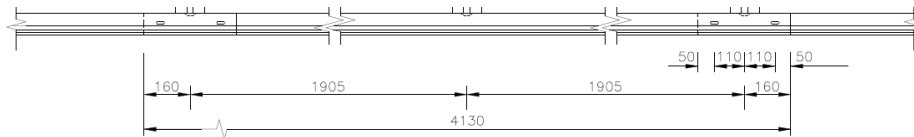
Figure 3: Plan view of guardrail, indicating lengths at slot placements
