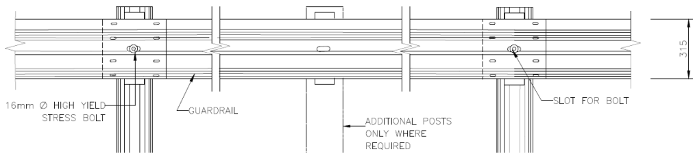
Figure 2: Side elevation, indicating slot placement
