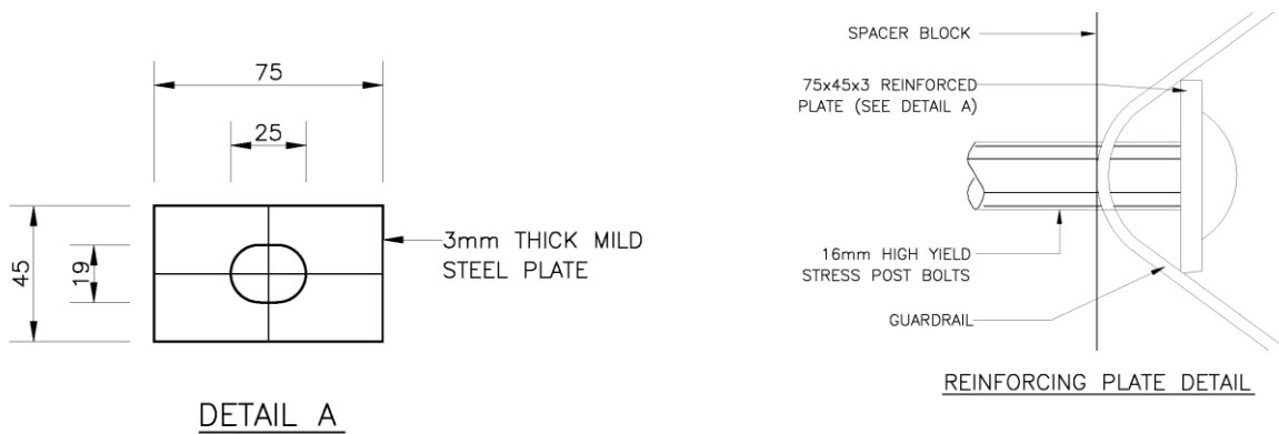
Figure 4: Reinforcing plate detail, see round headed stress bolt.
